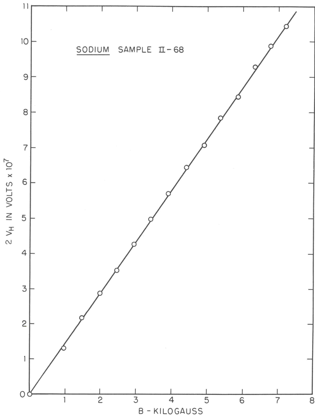
FIG. 3-1 HALL VOLTAGE \times 2 , 2V_H , VS. MAGNETIC FIELD. A.C. MEASUREMENTS
